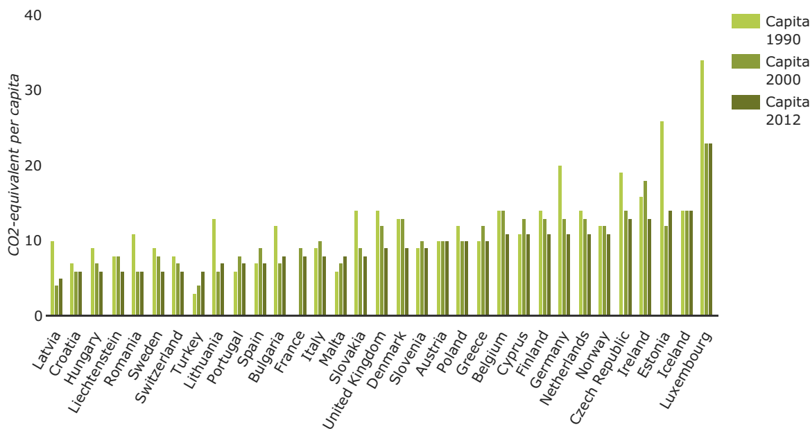
Figure 2: Greenhouse gas emissions per capita in EEA countries (1990, 2000 and 2012)
