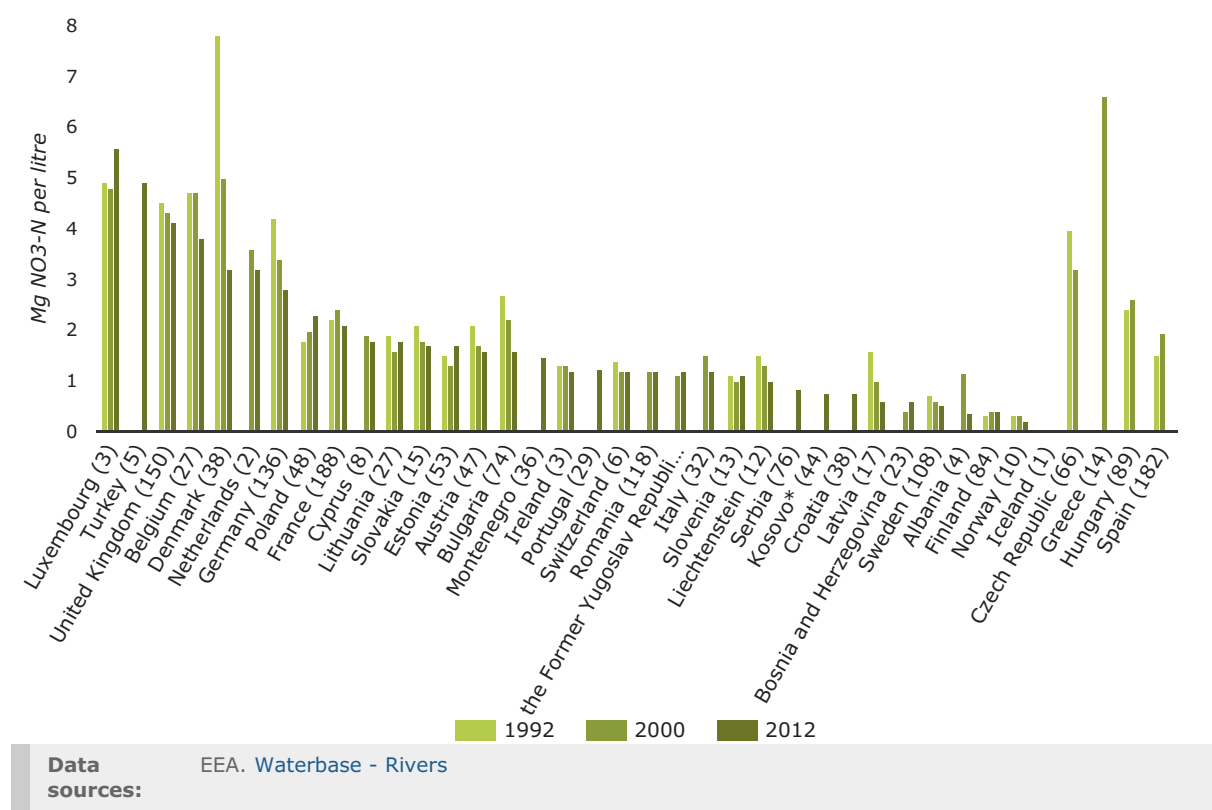
Figure 1: Average concentration of nitrate-nitrogen in rivers in 38 European countries (1992, 2000 and 2012)
